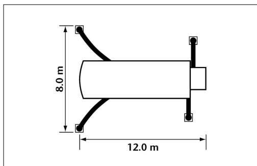
M40 – Mobile Concrete Boom Pump
